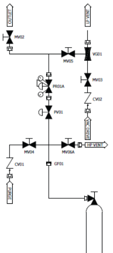
6-Valve
