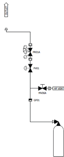
2-Valve
