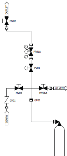
4-Valve
