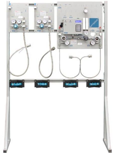
Symplcity™ UHP Auto-Switchover Panel with MicroLine™ UHP Manual Gas Panels mounted on a FastRack™.
